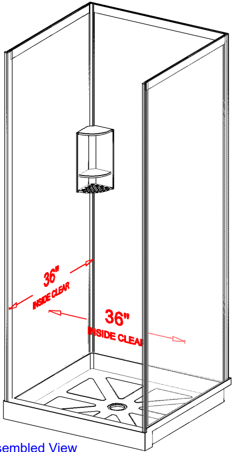
Assembled View
