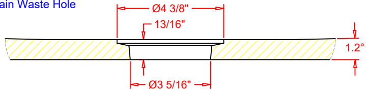
DETAIL 1 Drain Waste Hole
