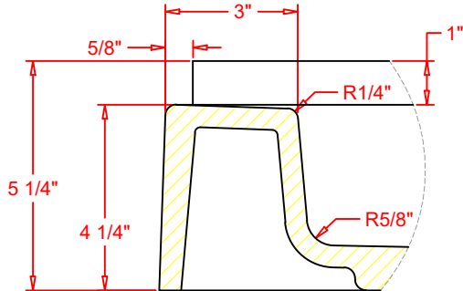
DETAIL 2 Front Threshold
