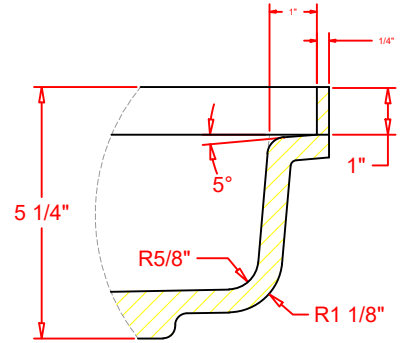
DETAIL 3 Water Dam / Panel Platform
