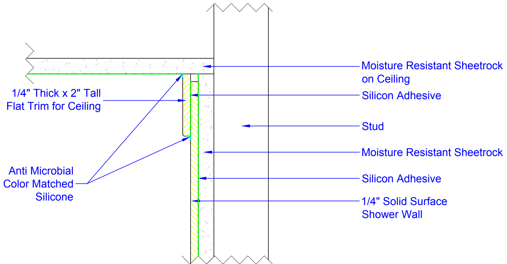
Typical cross section of flat trim at ceiling
