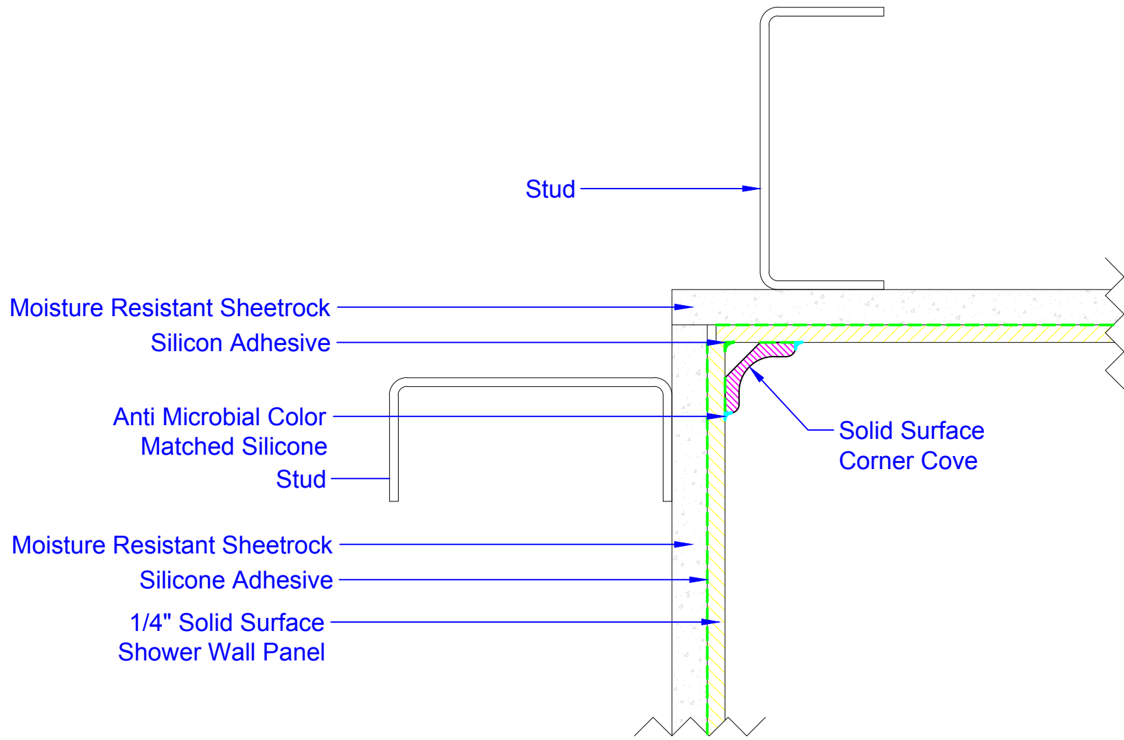
Typical plan view cross section of vertical cove trim
